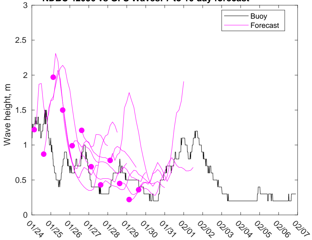
NDBC 42036 vs GFS Waves: 7 to 10 day forecast
