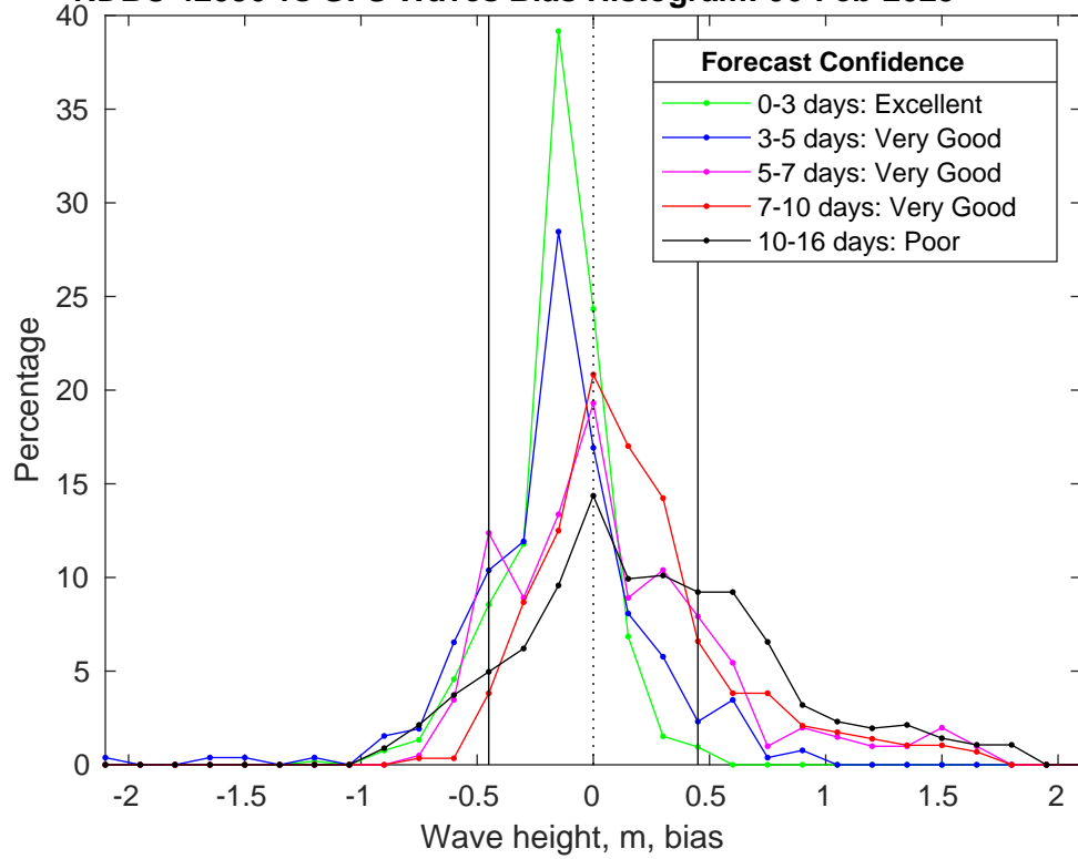
NDBC 42036 vs GFS Waves Bias Histogram: 06-Feb-2025
