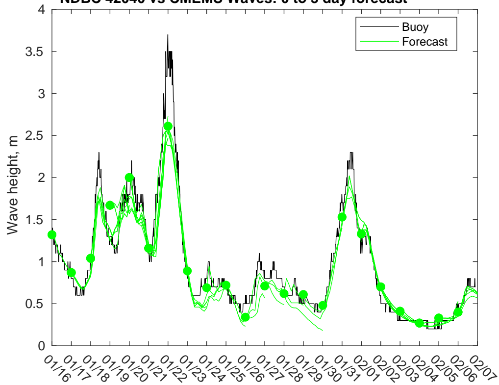
NDBC 42040 vs CMEMS Waves: 0 to 3 day forecast
