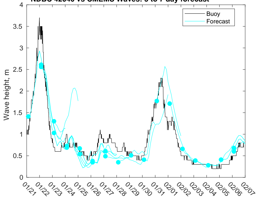
NDBC 42040 vs CMEMS Waves: 5 to 7 day forecast
