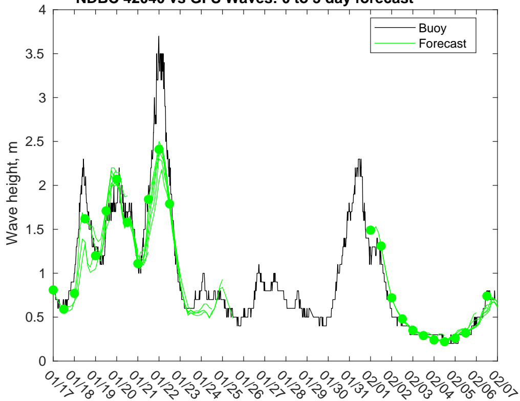
NDBC 42040 vs GFS Waves: 0 to 3 day forecast
