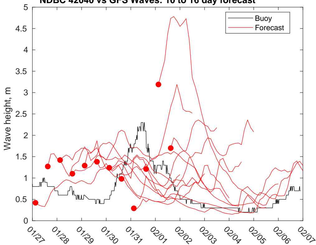
NDBC 42040 vs GFS Waves: 10 to 16 day forecast
