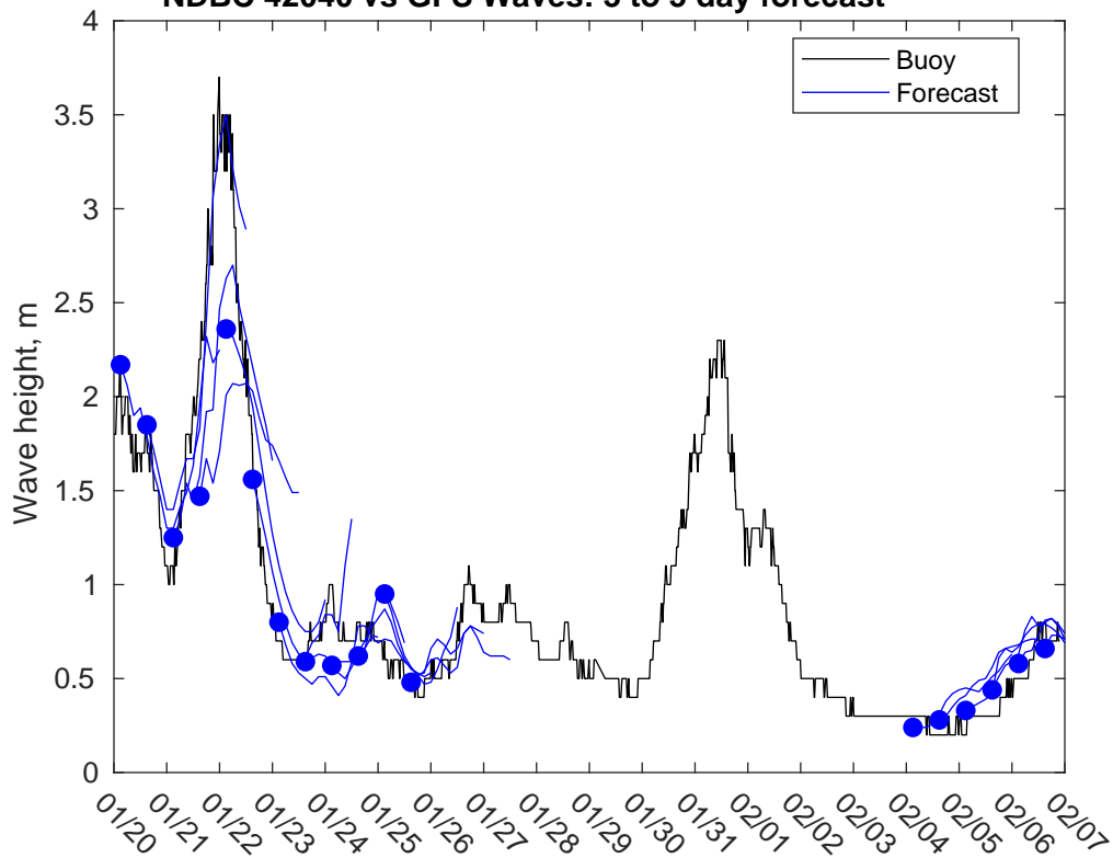
NDBC 42040 vs GFS Waves: 3 to 5 day forecast
