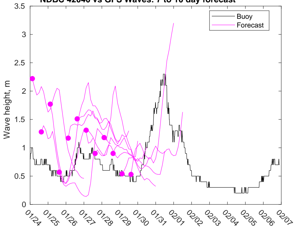
NDBC 42040 vs GFS Waves: 7 to 10 day forecast
