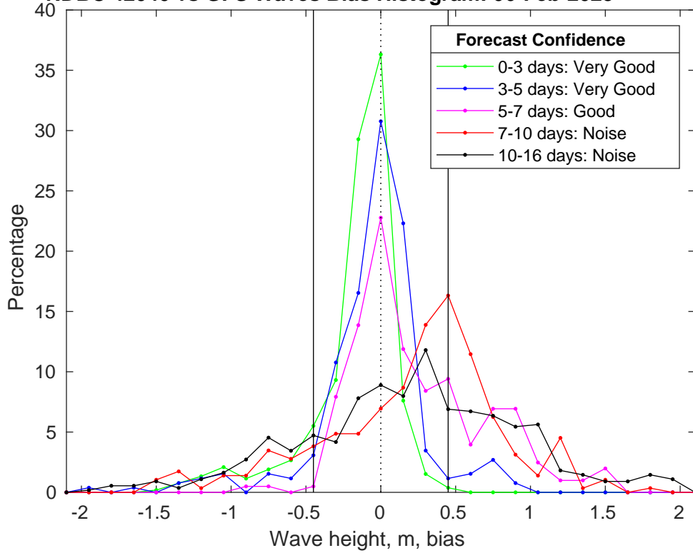
NDBC 42040 vs GFS Waves Bias Histogram: 06-Feb-2025
