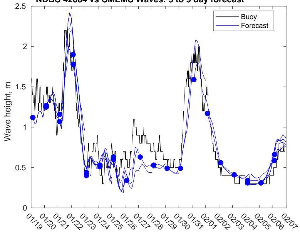
NDBC 42084 vs CMEMS Waves: 3 to 5 day forecast
