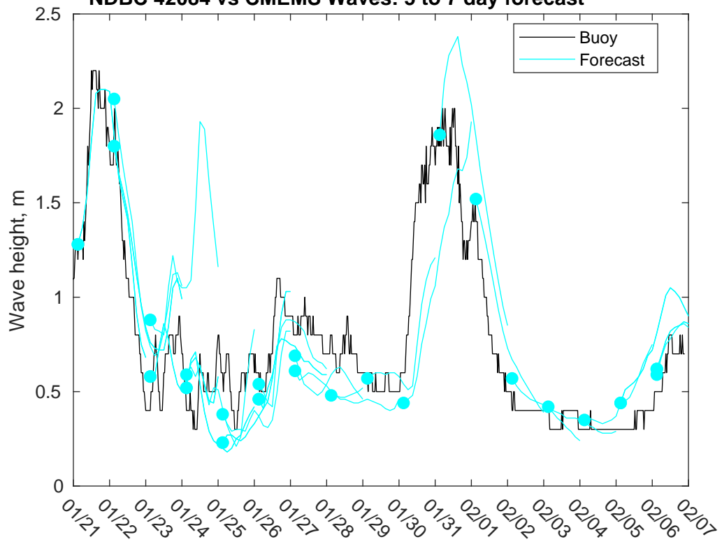
NDBC 42084 vs CMEMS Waves: 5 to 7 day forecast
