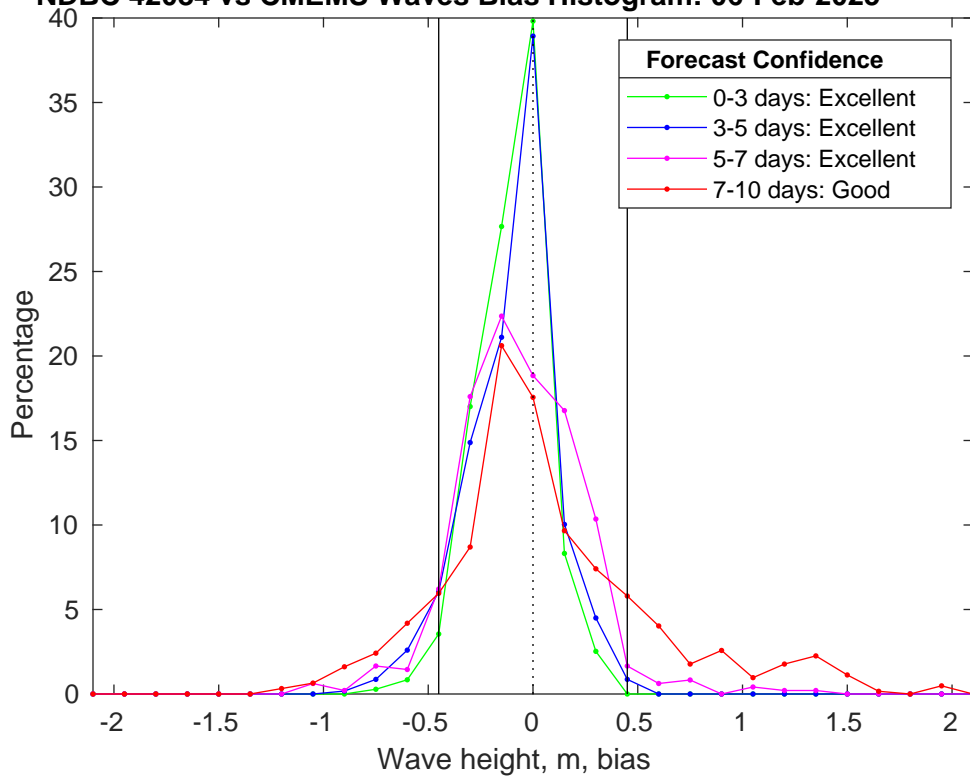
NDBC 42084 vs CMEMS Waves Bias Histogram: 06-Feb-2025
