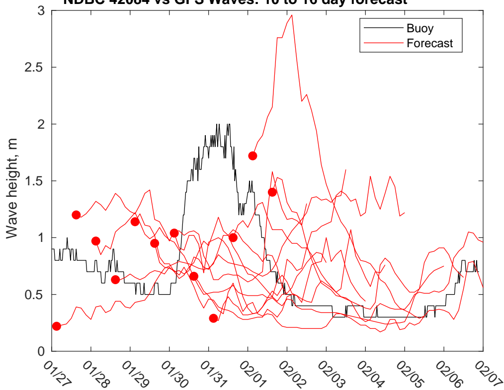
NDBC 42084 vs GFS Waves: 10 to 16 day forecast
