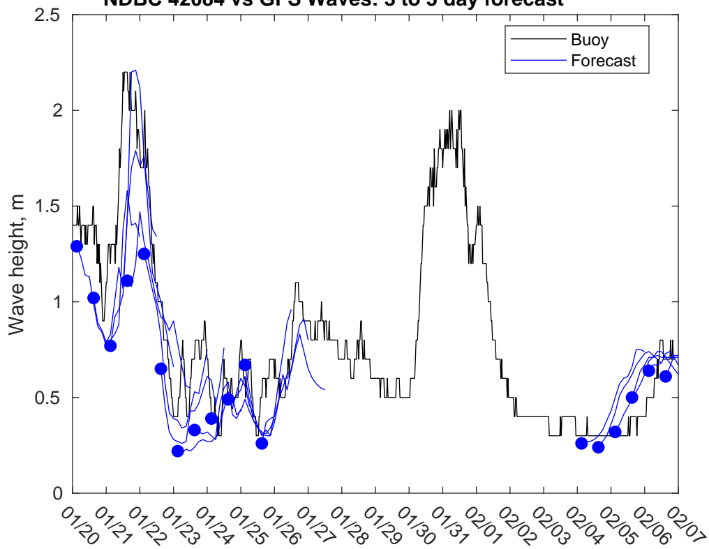
NDBC 42084 vs GFS Waves: 3 to 5 day forecast
