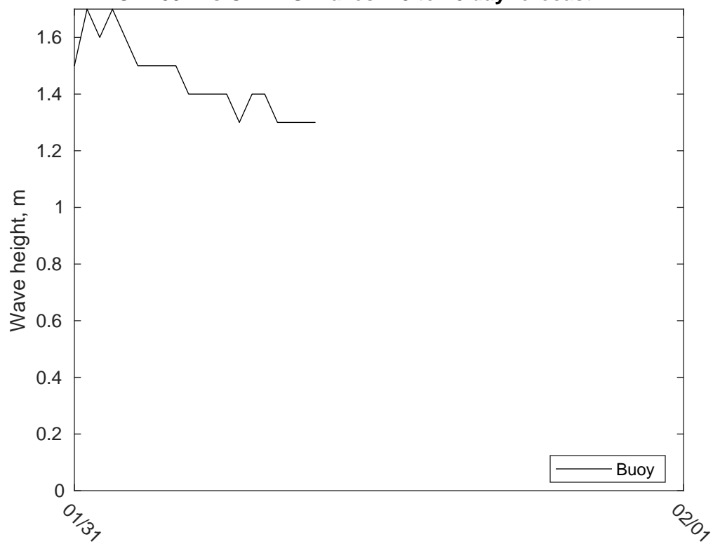
NDBC 42092 vs CMEMS Waves: 10 to 16 day forecast
