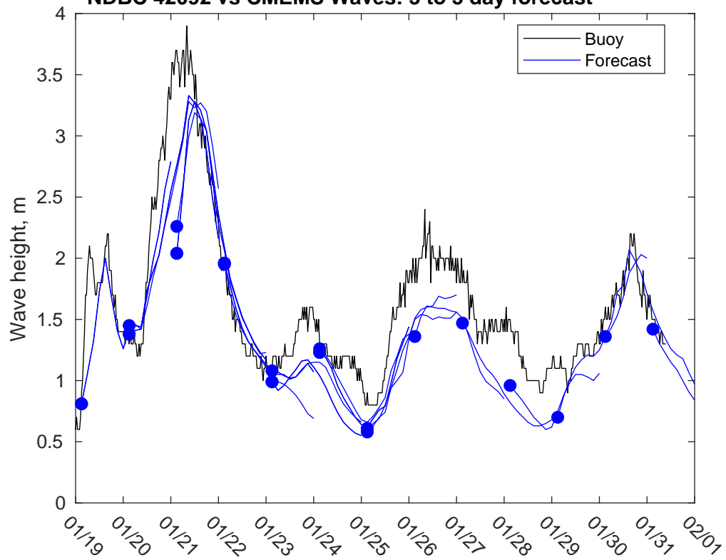
NDBC 42092 vs CMEMS Waves: 3 to 5 day forecast
