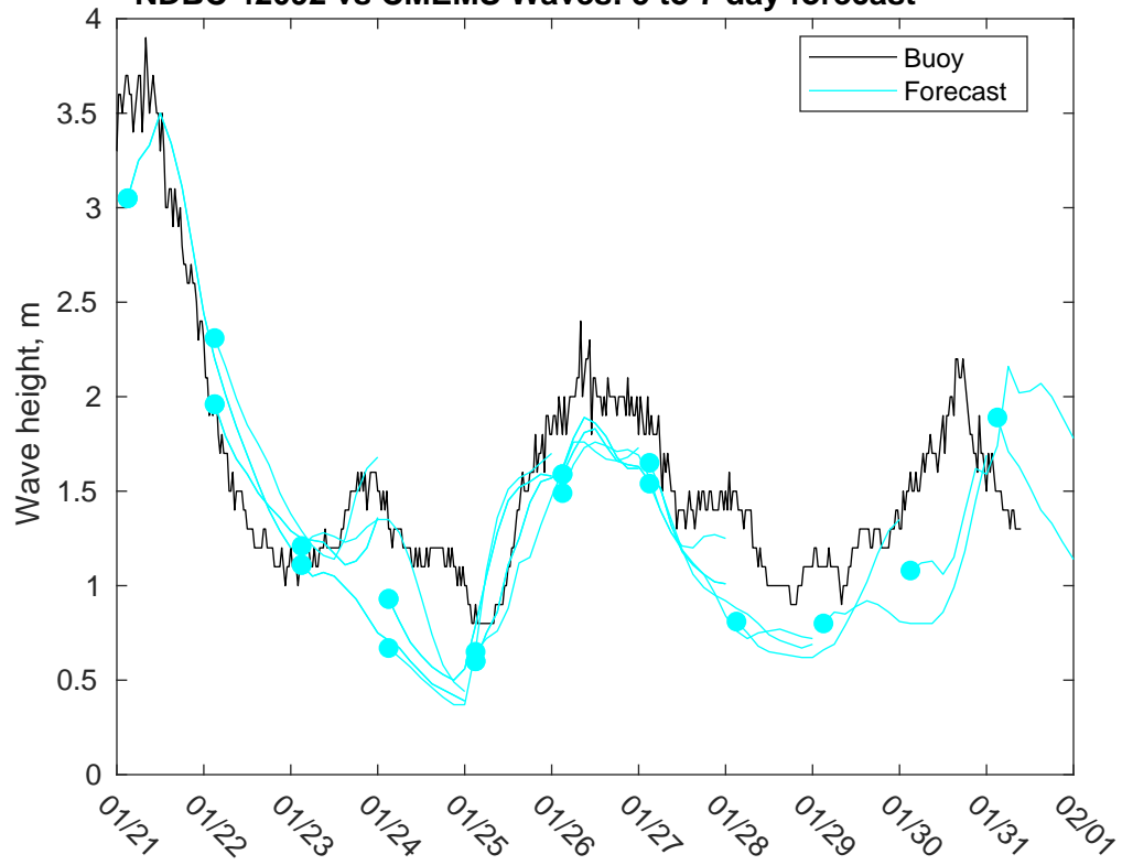
NDBC 42092 vs CMEMS Waves: 5 to 7 day forecast
