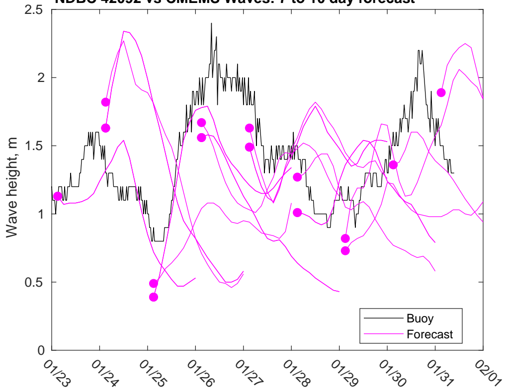
NDBC 42092 vs CMEMS Waves: 7 to 10 day forecast
