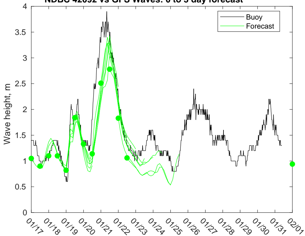
NDBC 42092 vs GFS Waves: 0 to 3 day forecast
