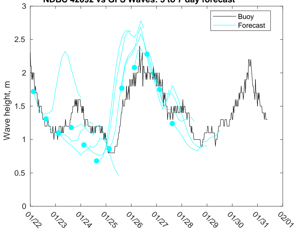
NDBC 42092 vs GFS Waves: 5 to 7 day forecast
