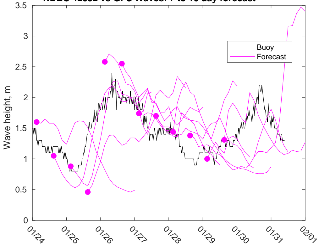
NDBC 42092 vs GFS Waves: 7 to 10 day forecast
