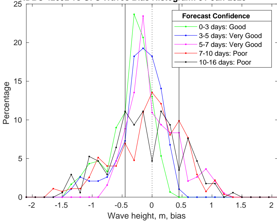
NDBC 42092 vs GFS Waves Bias Histogram: 31-Jan-2025
