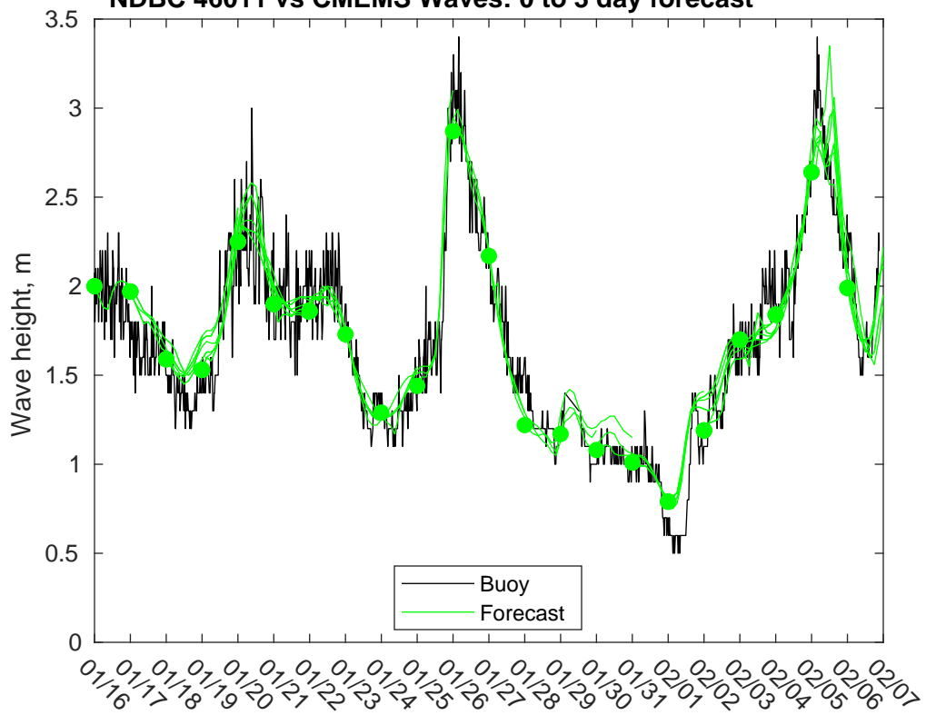
NDBC 46011 vs CMEMS Waves: 0 to 3 day forecast
