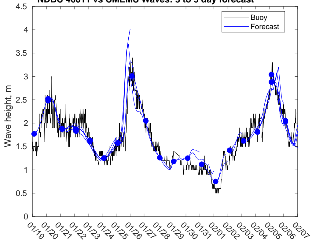
NDBC 46011 vs CMEMS Waves: 3 to 5 day forecast
