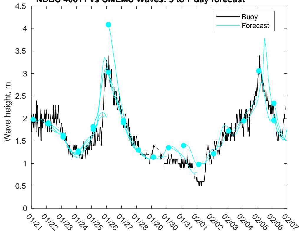
NDBC 46011 vs CMEMS Waves: 5 to 7 day forecast
