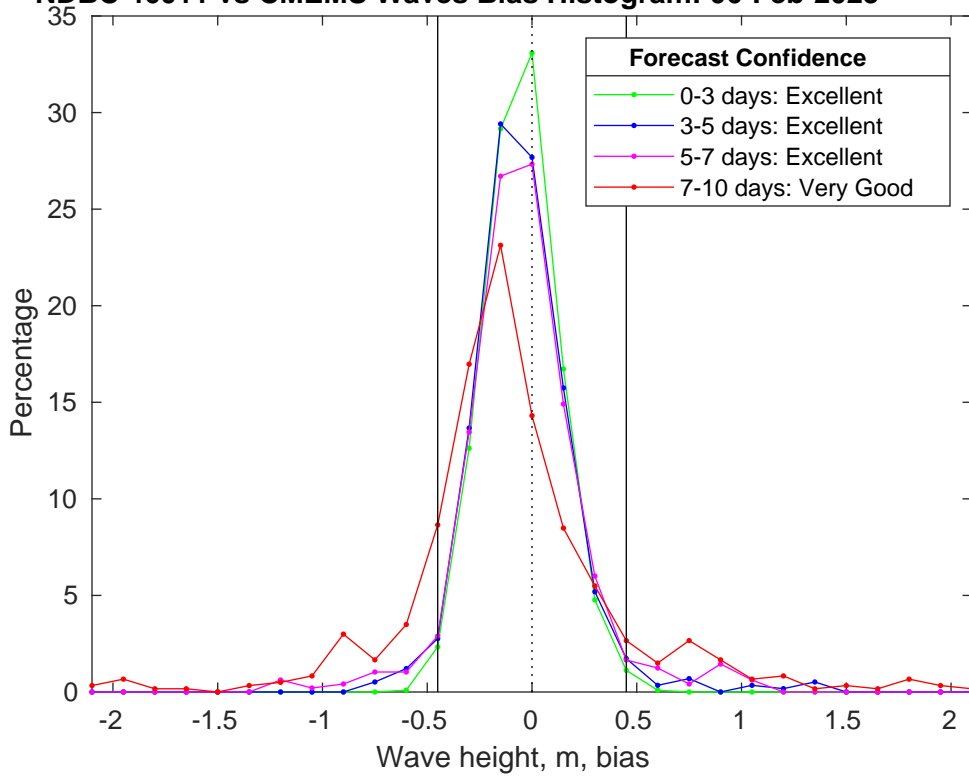
NDBC 46011 vs CMEMS Waves Bias Histogram: 06-Feb-2025
