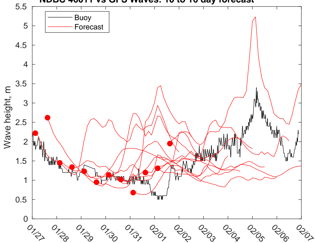
NDBC 46011 vs GFS Waves: 10 to 16 day forecast
