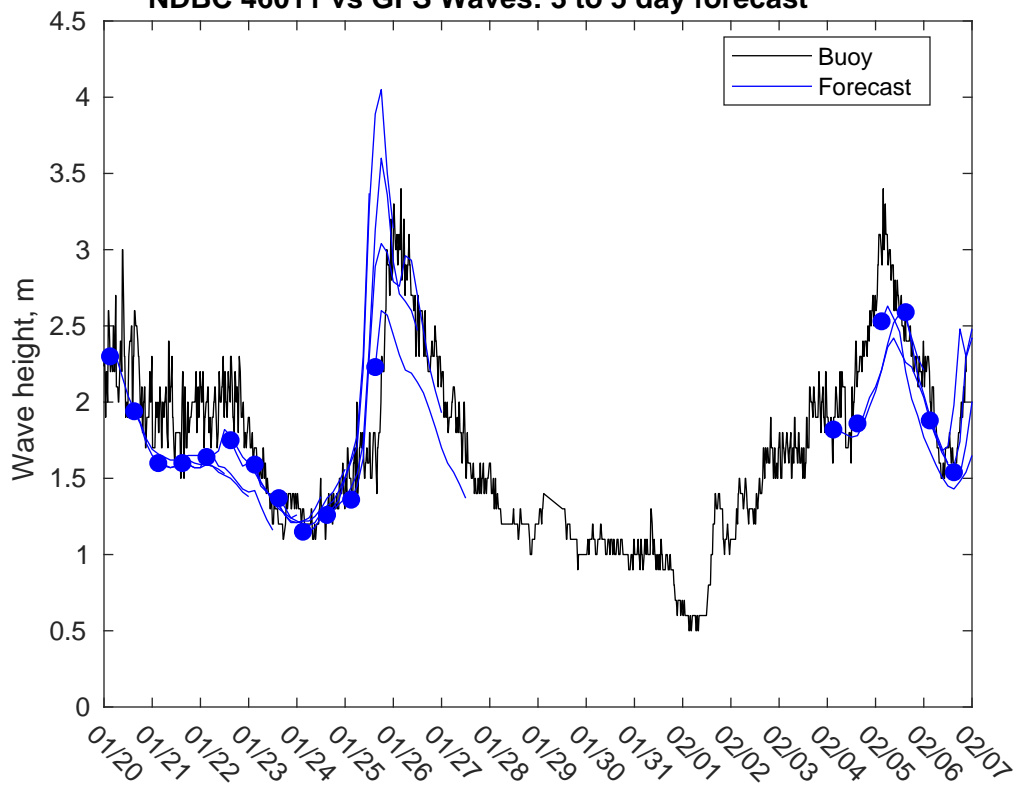
NDBC 46011 vs GFS Waves: 3 to 5 day forecast
