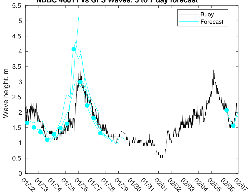
NDBC 46011 vs GFS Waves: 5 to 7 day forecast
