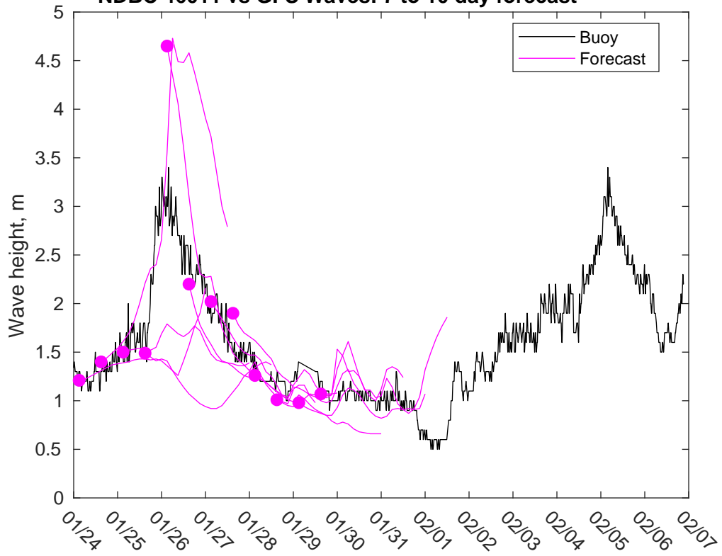
NDBC 46011 vs GFS Waves: 7 to 10 day forecast
