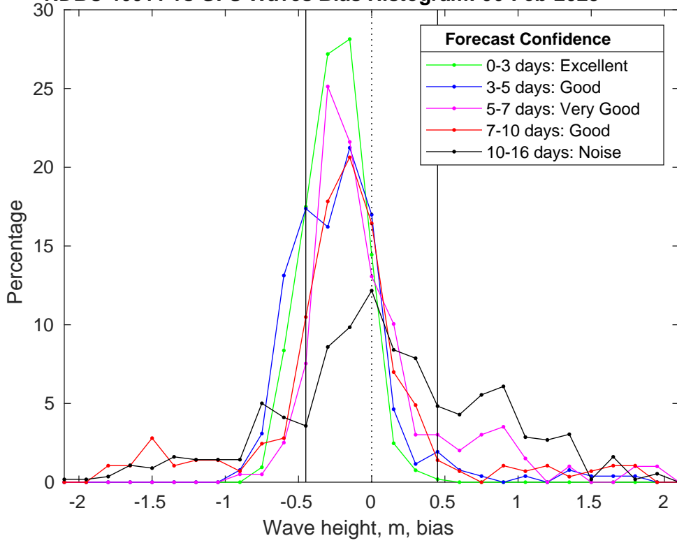
NDBC 46011 vs GFS Waves Bias Histogram: 06-Feb-2025
