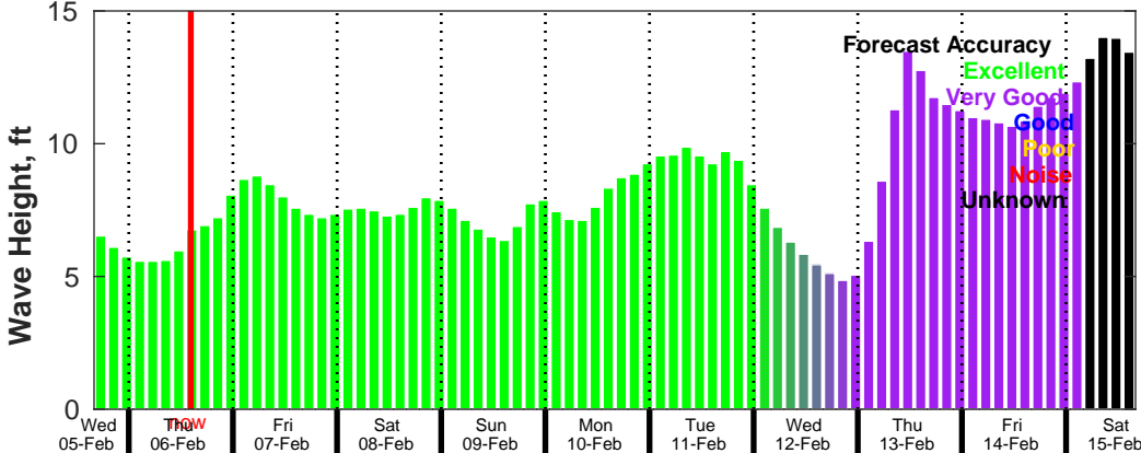
CMEMS Wave Forecast for NDBC 46011 from 05-Feb-2025 16:00:00 to 15-Feb-2025 16:00:00
