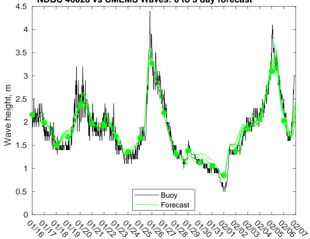
NDBC 46028 vs CMEMS Waves: 0 to 3 day forecast
