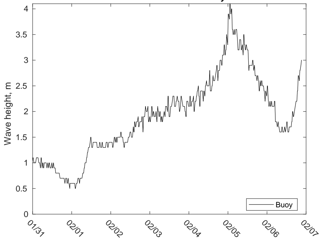
NDBC 46028 vs CMEMS Waves: 10 to 16 day forecast
