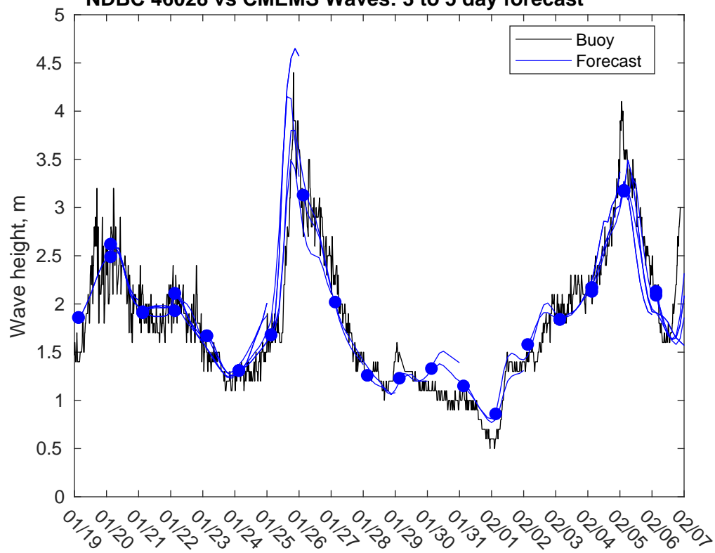
NDBC 46028 vs CMEMS Waves: 3 to 5 day forecast
