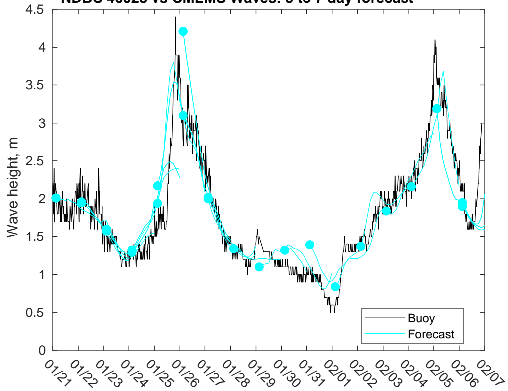
NDBC 46028 vs CMEMS Waves: 5 to 7 day forecast
