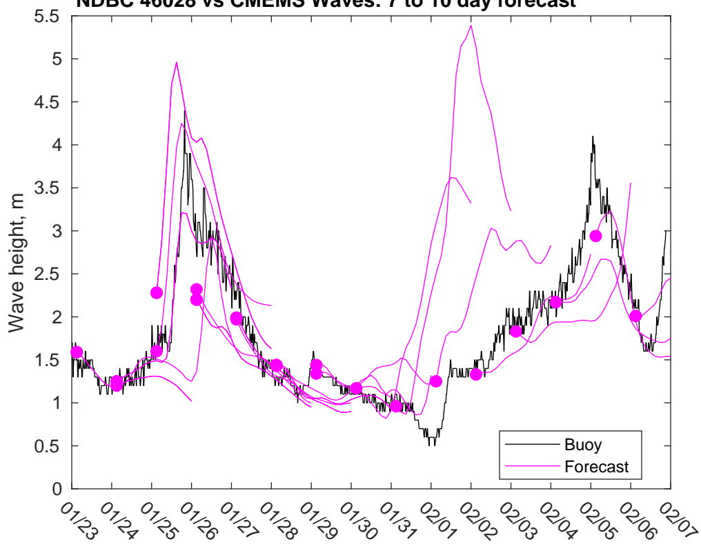
NDBC 46028 vs CMEMS Waves: 7 to 10 day forecast
