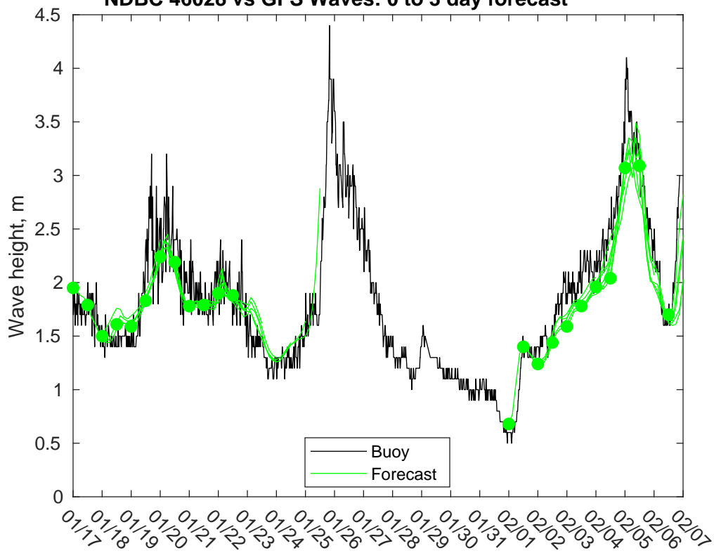
NDBC 46028 vs GFS Waves: 0 to 3 day forecast
