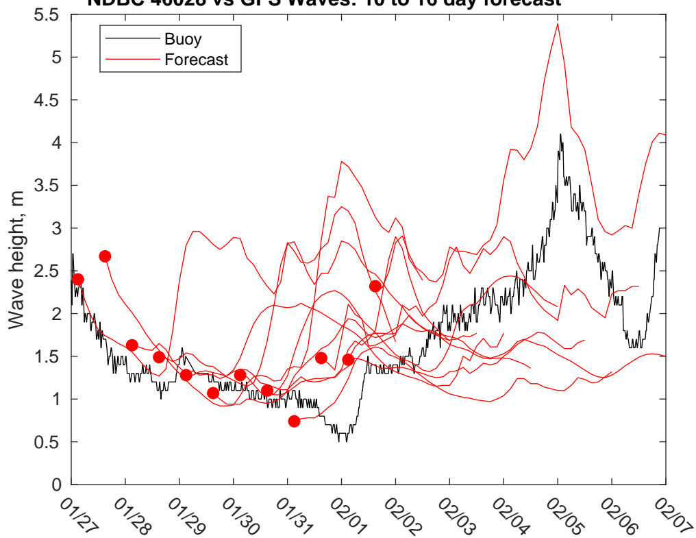
NDBC 46028 vs GFS Waves: 10 to 16 day forecast
