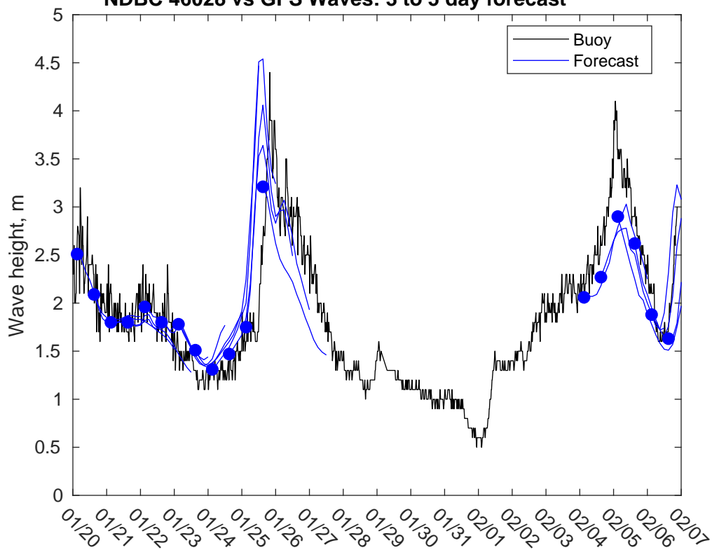
NDBC 46028 vs GFS Waves: 3 to 5 day forecast
