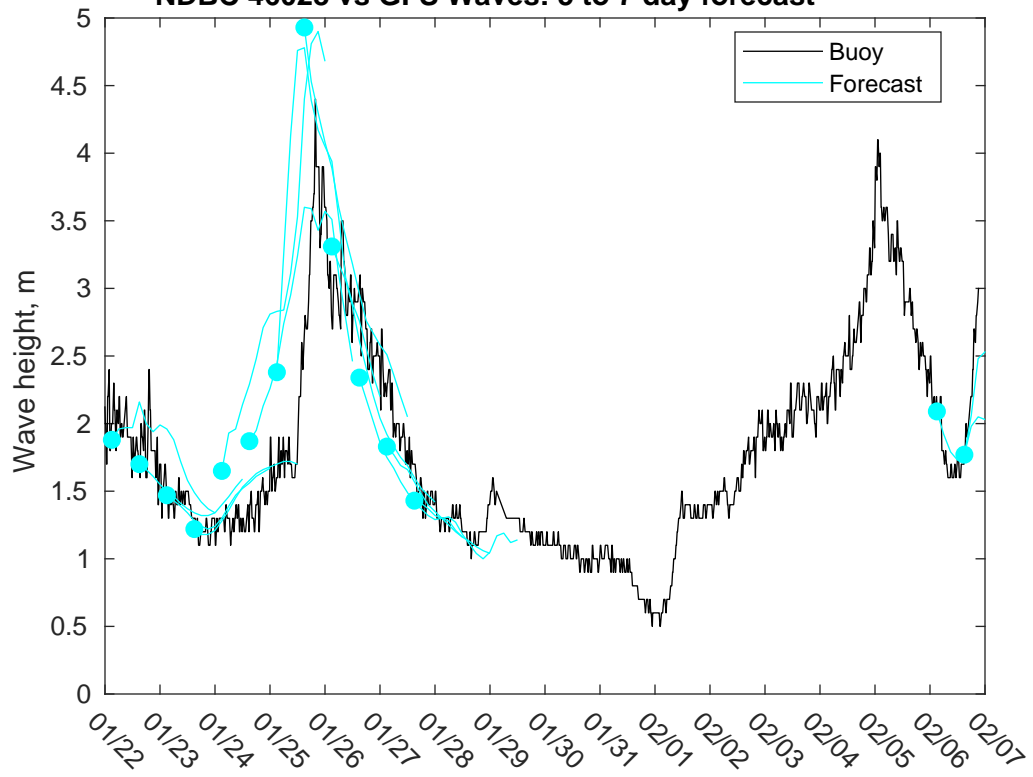
NDBC 46028 vs GFS Waves: 5 to 7 day forecast
