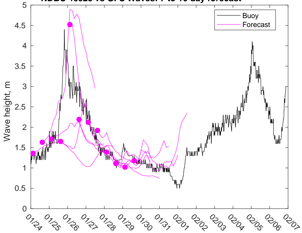
NDBC 46028 vs GFS Waves: 7 to 10 day forecast
