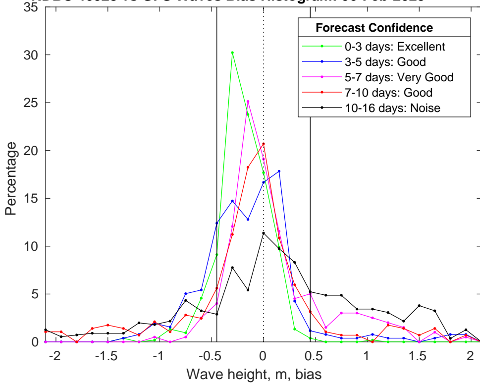
NDBC 46028 vs GFS Waves Bias Histogram: 06-Feb-2025
