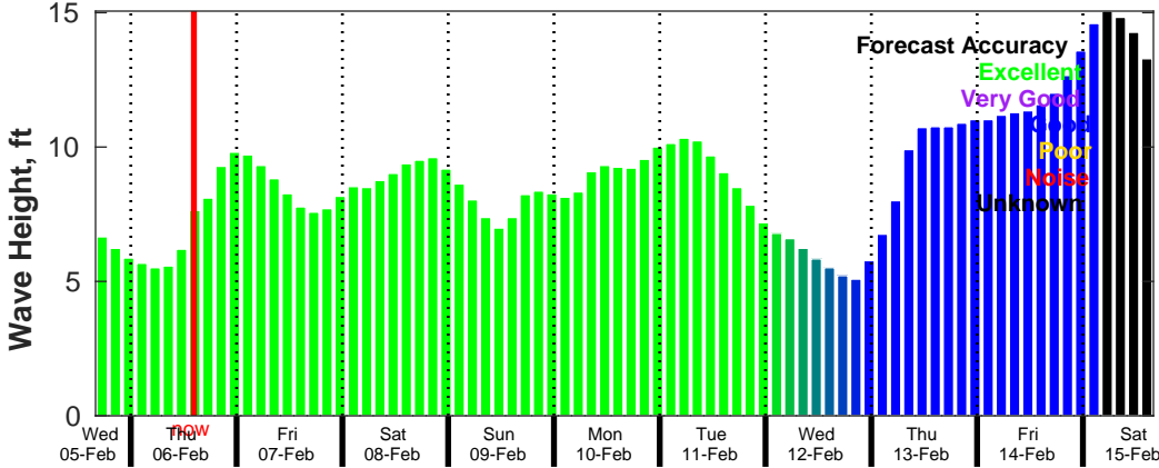
CMEMS Wave Forecast for NDBC 46028 from 05-Feb-2025 16:00:00 to 15-Feb-2025 16:00:00
