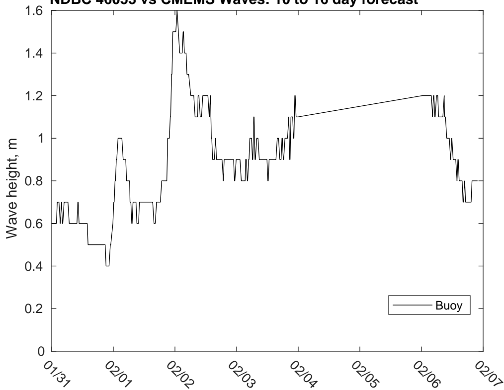
NDBC 46053 vs CMEMS Waves: 10 to 16 day forecast
