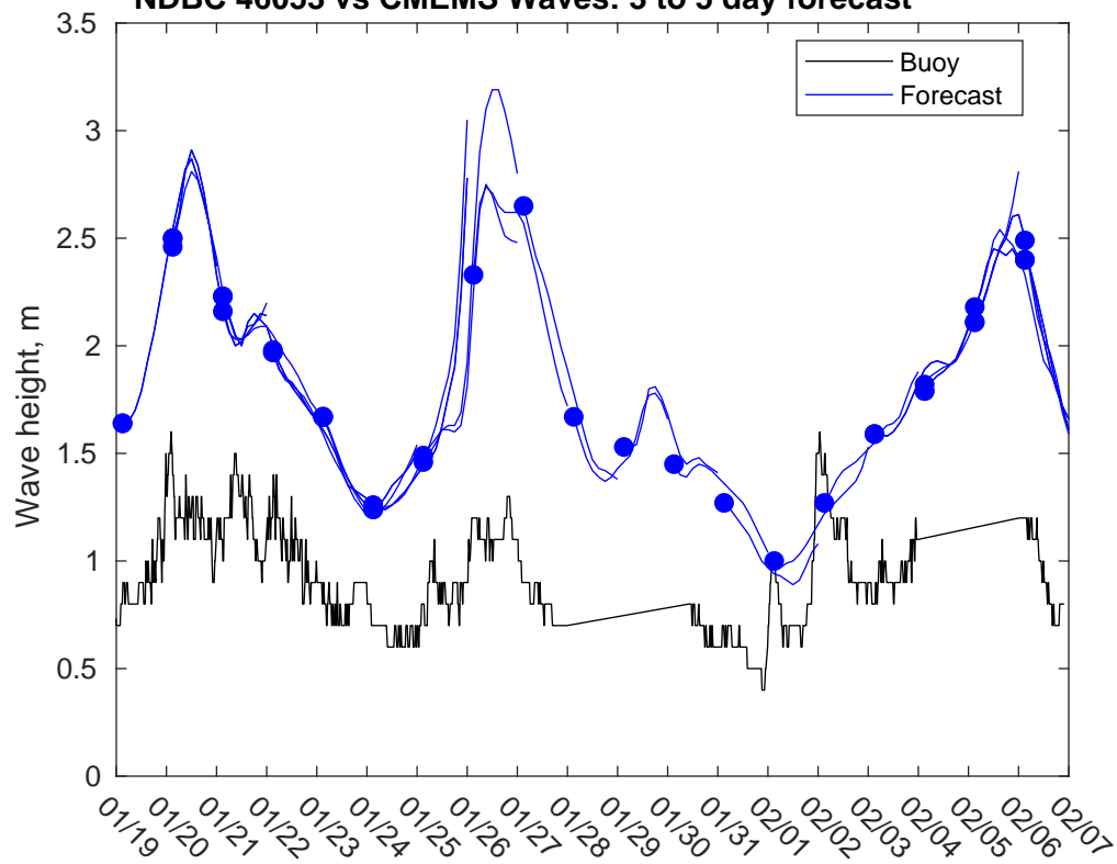
NDBC 46053 vs CMEMS Waves: 3 to 5 day forecast
