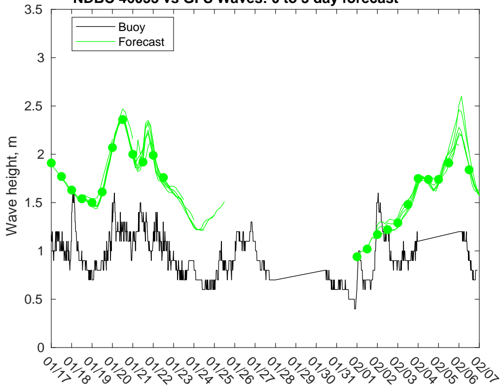
NDBC 46053 vs GFS Waves: 0 to 3 day forecast
