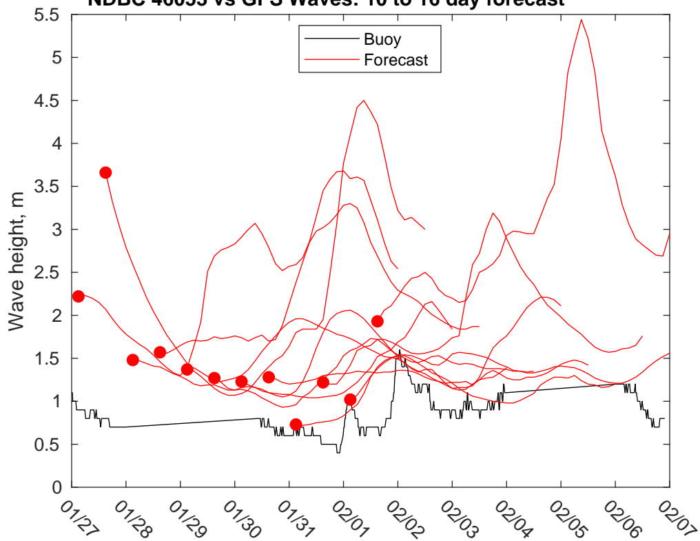
NDBC 46053 vs GFS Waves: 10 to 16 day forecast
