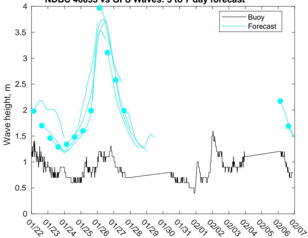
NDBC 46053 vs GFS Waves: 5 to 7 day forecast
