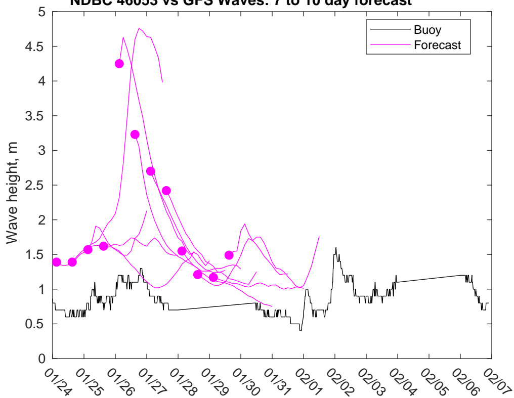
NDBC 46053 vs GFS Waves: 7 to 10 day forecast
